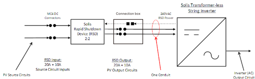
Figure 3.1 System diagram
